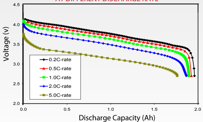
CELL DISCHARGE CURVE AT DIFFERENT DISCHARGE RATE
