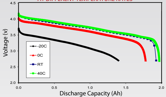
CELL DISCHARGE CURVE AT DIFFERENT TEMPERATURE RATES
